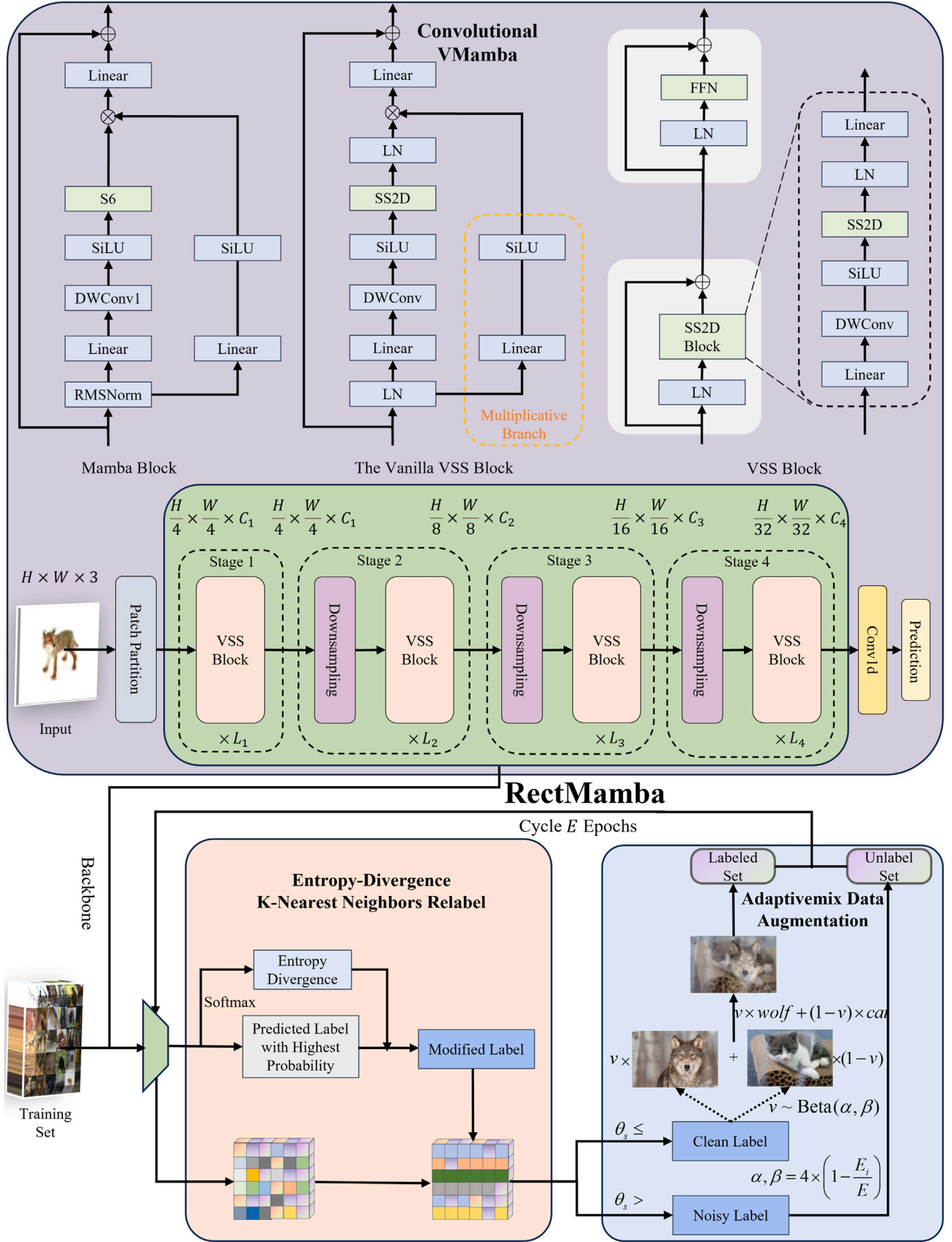
Fig. 2. Overview of RectMamba framework which includes: the CVMamba for tackling the warm-up phase during pre-training; the EDKR for noisy label correction; and the Adaptivemix method for adjustable data augmentation intensity throughout training epochs. Note: The Mamba block (left) shows the original S6-based design for comparison only. All actual vision components (Vanilla VSS Block, VSS Block, CVMamba) use SS2D instead of S6.
