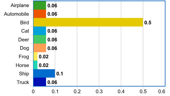
Fig. 5. This image displays predicted probability values with a higher entropy (2.5191), yet the clear separation between the top two predicted probabilities (Bird category) signifies that the model has a high level of confidence in this prediction.
