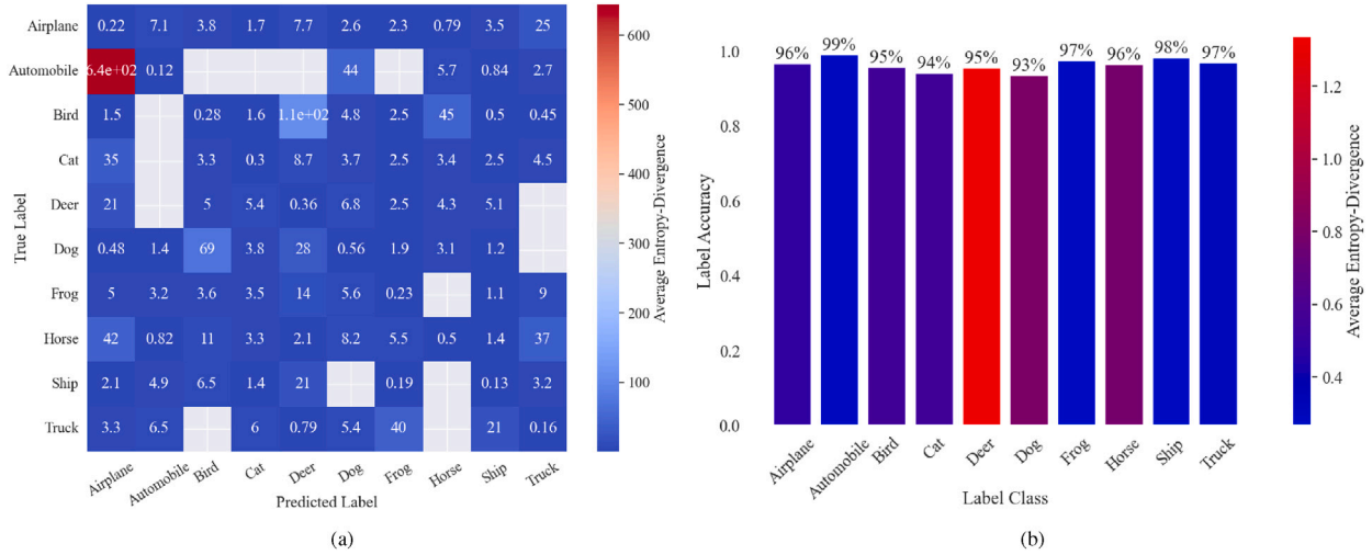
Fig. 1. On the left, a heatmap compares the average entropy-divergence values between predicted and true labels. Darker red shades indicate higher entropy values, with x-axis showing predicted categories and y-axis representing true categories. On the right, the post-correction accuracy by class is depicted. Darker blue bars indicate lower model uncertainty and lower entropy.
