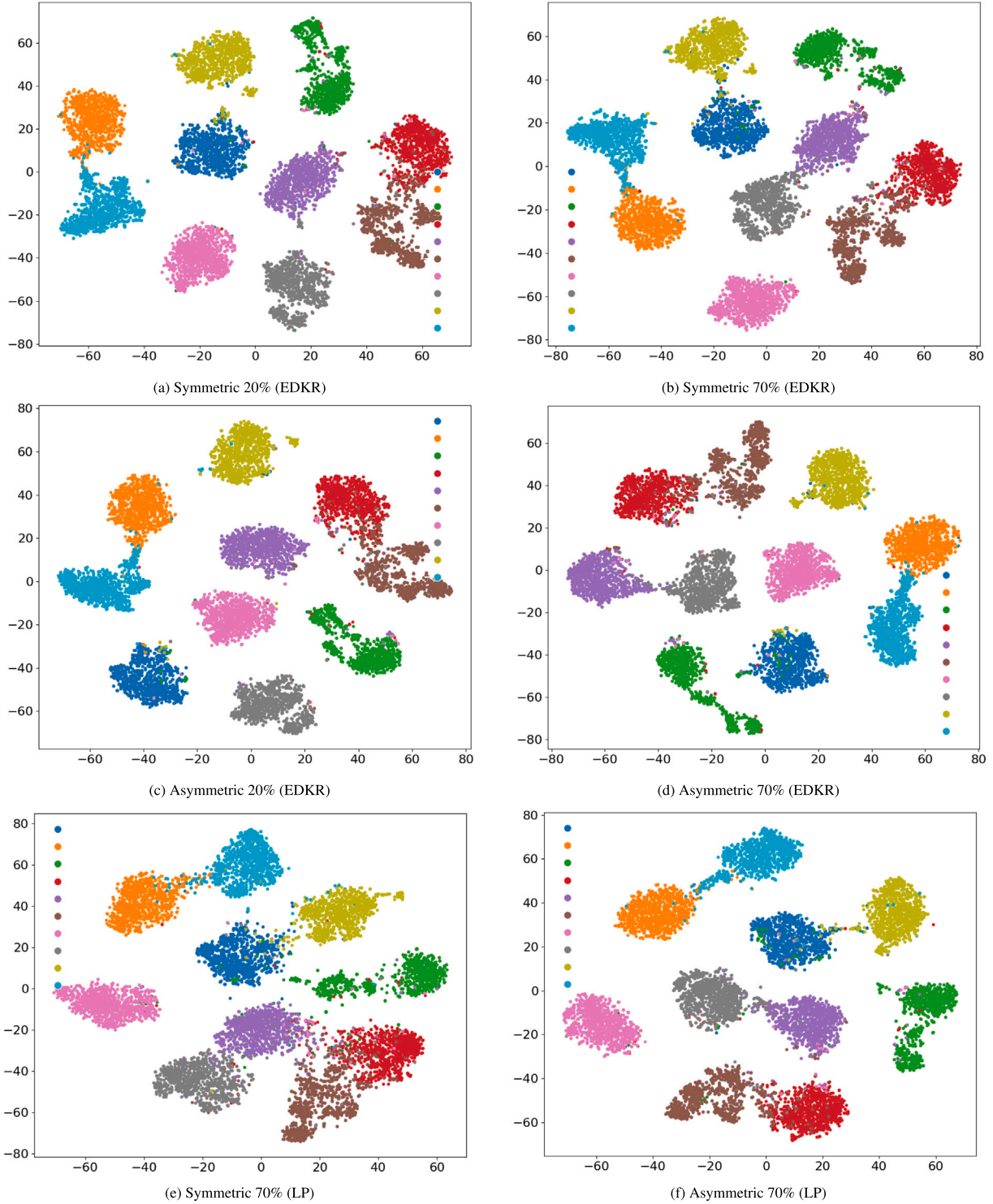
Fig. 7. T-SNE visualizations of test features from the CIFAR-10 dataset under different noise settings after 50 epochs of training. Subfigures (a)–(d) show results using RectMamba with EDKR under symmetric and asymmetric noise at 20 % and 70 %. Subfigures (e) and (f) show results of a controlled variant, where the EDKR module is replaced with Label Propagation (LP) under 70 % symmetric and asymmetric noise, respectively. Each of the ten classes— Airplane , Automobile , Bird , Cat , Deer , Dog , Frog , Horse , Ship , Truck —is distinctly represented by a unique color: deep blue, vibrant orange, grassy green, bold red, muted purple, earthy brown, soft pink, medium grey, bright lime green, and clear aqua, respectively.
