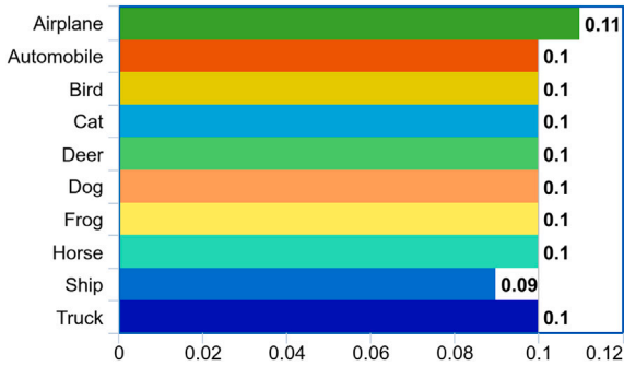
Fig. 3. This image displays multiple class prediction probabilities, with no single class dominating. This results in a high entropy value (3.3205), indicating that the model is unsure about the correct label.
