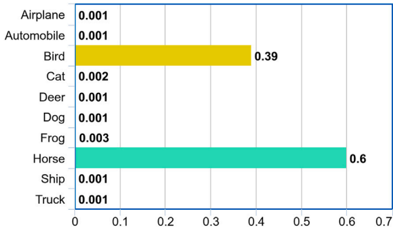
Fig. 4. This image shows a clear peak in predicted probability for one class, resulting in low entropy (1.0656), which signifies high confidence in the prediction. The model predicts the class 'Horse' with a high level of certainty. Although the model shows certainty, the close values between the top two predictions indicate a moderate confidence level in the prediction.
