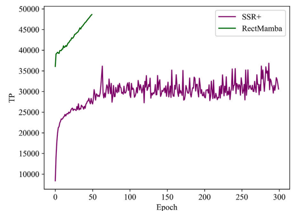
Fig. 6. Comparative analysis of label refine performance between RectMamba over 50 epochs and SSR + over 300 epochs.
